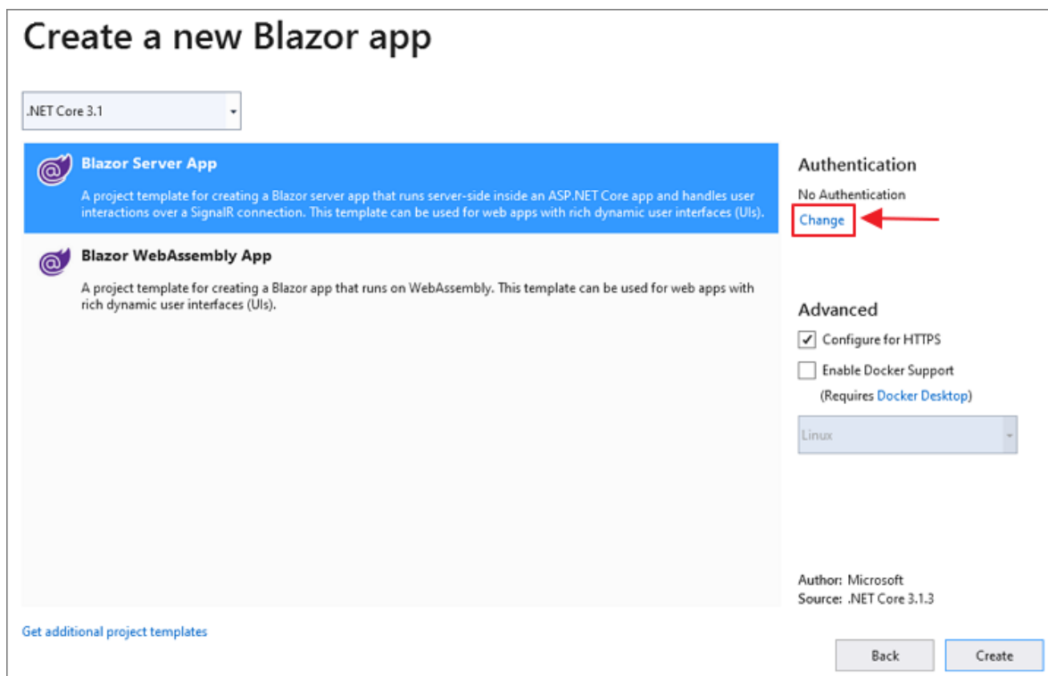
Figure 23: Change Authentication
