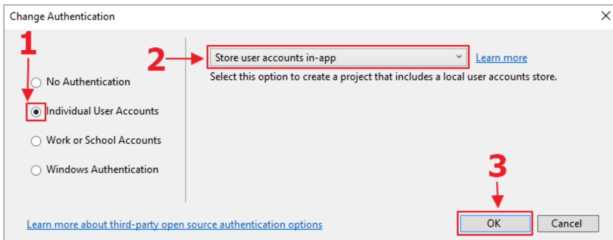
Figure 24: Set Authentication
