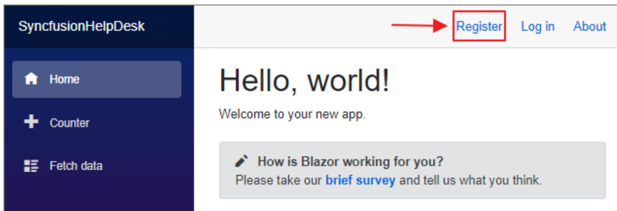
Figure 30: Register User
