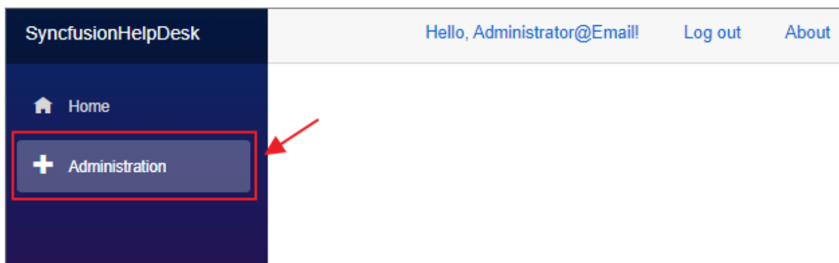
Figure 58: Administration Link
